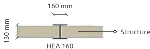
Section A-A' / Plan view M 1:20
